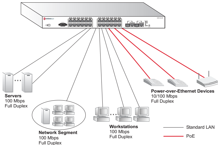
Figure 2-1. Collapsed Backbone
